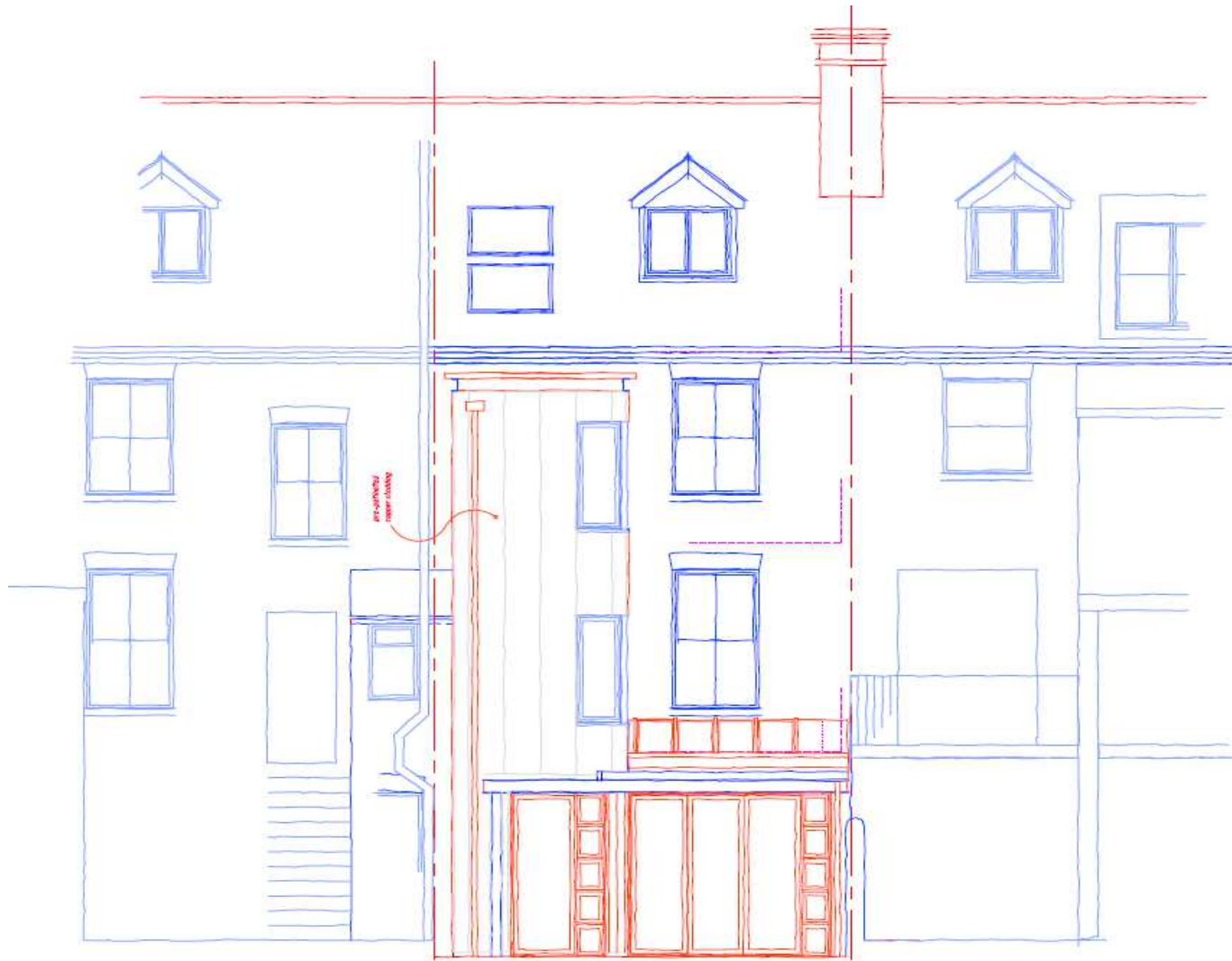
Rear elevation
